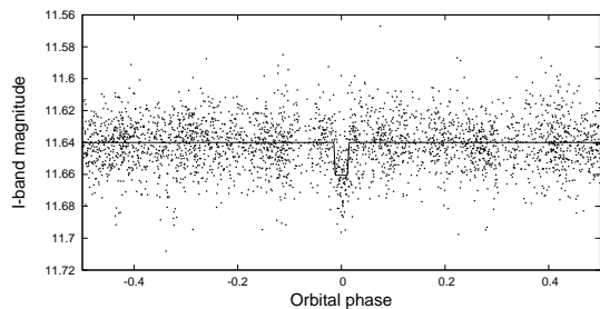
FIG. 1.— The unbinned light curve of HAT-P-12 including all 2927 instrumental I band 5.5-min cadence measurements obtained with the HAT-5 (Arizona) telescope of HATNet (see text for details), and folded with the period of P = 3.2130598 days (which is the result of the fit described in § 3).
