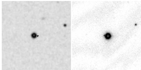
FIG. 6.— Images of a 2''.5 \times 2''.5 field containing HAT-P-12 from the POSS-I Red survey (Left), and from our FLWO 1.2 m z band follow-up observations (Right, see section 2.4). The dates of the exposures are 1955 April 13 and 2009 February 5 respectively. The cross marks the position of HAT-P-12 in 1955 and the triangle marks the position in 2009. Between these two dates HAT-P-12 moved \sim 7''.5 to the west. From the POSS-I image we can rule out stars brighter than R \sim 19 at the current position of HAT-P-12.
